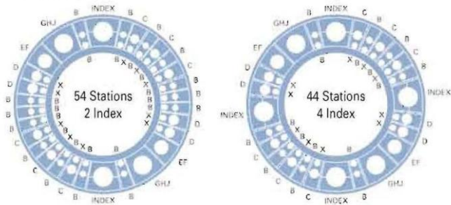
Turret Layout
